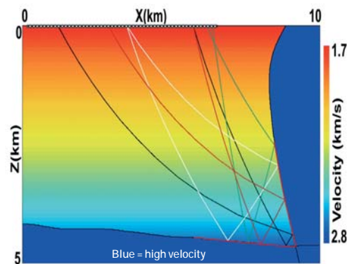
Fig. 2: The prismatic reflections provide precious information about the overhanging parts of the diapirs.
