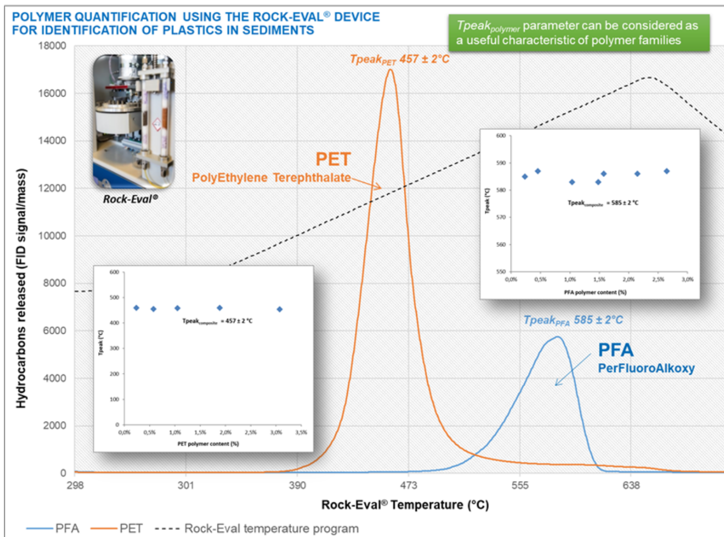
Image: Rock-Eval® thermograms illustrating the Tpeak for PET and PFA polymers
