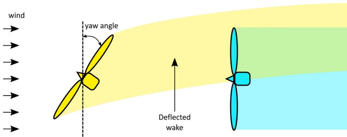
Figure 2: Wake realignment with yaw control
