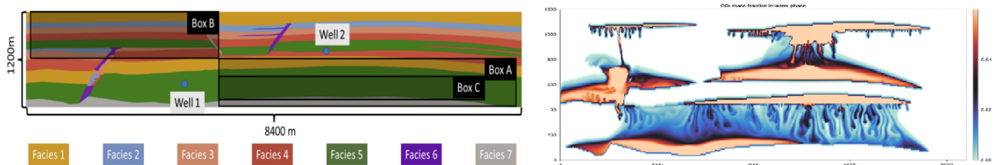
Figure 1: Distribution of lithological facies in the reservoir and locations of injection wells Well1 and Well2 (left), final distribution of CO 2 dissolved in water as calculated by the IFPEN simulator: Geoxim (right)
