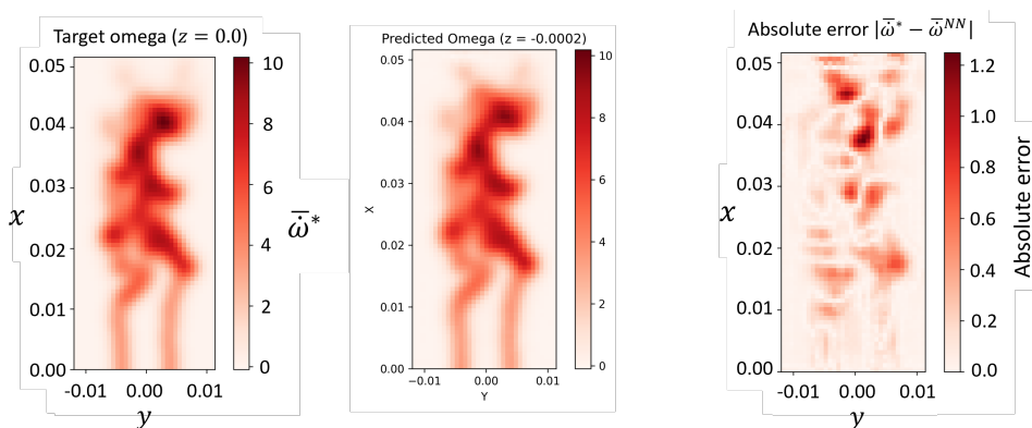
Figure 1: Comparison of the omega hydrogen reaction rate (mol/s) between a reference solution (left) and a field predicted by a CNN (center). The absolute error between the two fields is shown on the right.
