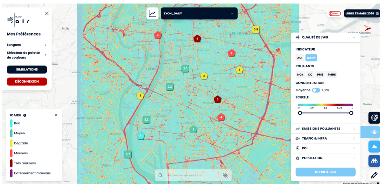
Figure 1: Street-level representation of the air quality index in the Lyon metropolitan area: simulated concentrations using virtual sensors (represented by pentagons) generated by the PLANET'AIR platform and values provided by monitoring stations located throughout the area (represented by squares).
