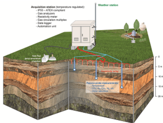
Leak detection in the vadose zone - Natural CO2 emission variation: soil breathing
