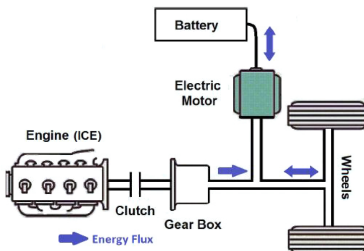
Energy flow in a hybrid vehicle, to be controlled by the onboard management system.
