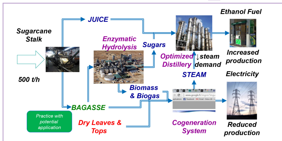
Diagram showing an ethanol production and heat/electricity cogeneration process.
